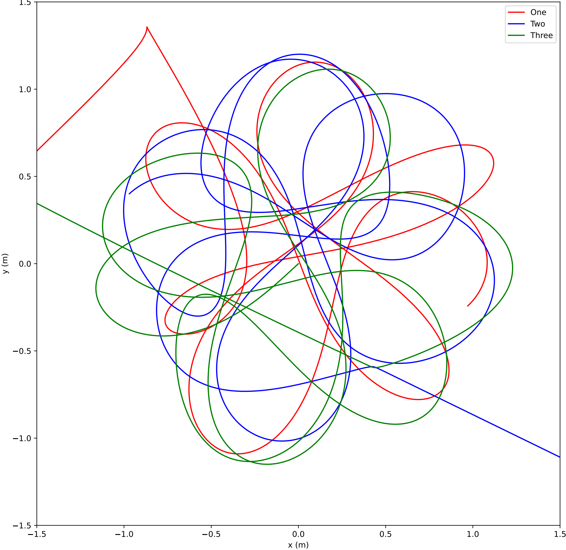
Unstable Three-Body Trajectory Integrated with the Symplectic Euler Method
